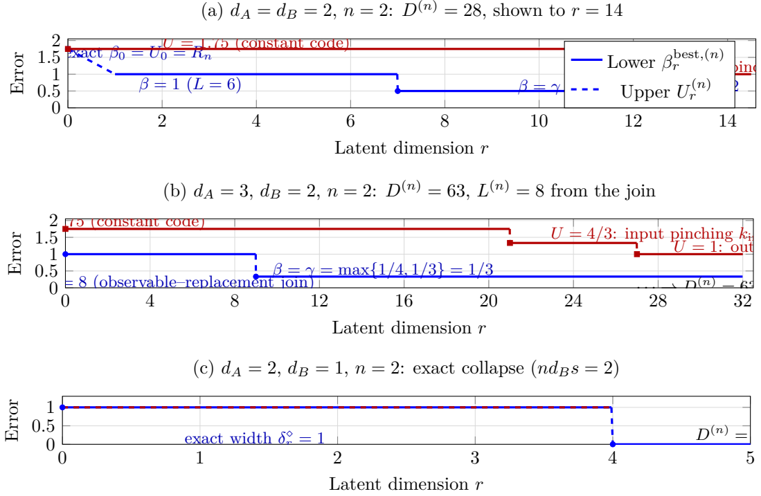
Figure 2: Certified lower and upper envelopes of the instrument compression width. (a) The worked example d_A = d_B = 2, n = 2 (Example 6.2): the upgraded value \beta_0 = R_n = 1.75 at r = 0 (exact, meeting the upper envelope) and \beta_r^{\text{best},(n)} = 1 for 1 \leq r \leq 6 , with \gamma = \max\{\rho_n, 1/d_A\} = 1/2 for 7 \leq r < 28 ; the upper envelope is R_{\text{inst}} = 1.75 for 0 \leq r < 12 and 1 from balanced two-sector output pinching for 12 \leq r \leq 14 , while convex projection exceeds 1.75 throughout and input pinching enters at r_{\text{in}} = 14 with the same value 1. (b) d_A = 3, d_B = 2, n = 2 : the one-sphere dimension L^{(n)} = 8 comes from the observable-replacement join; the upper envelope steps down 1.75 \rightarrow 4/3 \rightarrow 1 at r = 21 (three-block input pinching) and r = 27 (two-block output pinching), and the intermediate lower bound is \gamma = 1/3 . (c) The exact collapse for d_A = 2, d_B = 1, n = 2 (Theorem 5.18): both envelopes equal the exact width, which is 1 below D^{(n)} = 4 and 0 from D^{(n)} on. Filled circles and squares mark the lower and upper envelopes in (a) and (b); dashed segments mark the jumps.
